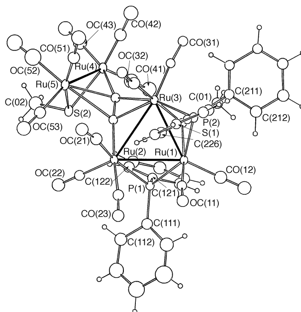
Fig. 1 Plot of a molecule of [\text{Ru}_5(\mu_4\text{-C}_2)(\mu\text{-SMe})_2(\mu\text{-PPh}_2)_2(\text{CO})_{13}] 2 showing the atom numbering scheme. In both figures, non-hydrogen atoms are shown as 20% thermal ellipsoids; hydrogen atoms have arbitrary radii of 0.1 Å
