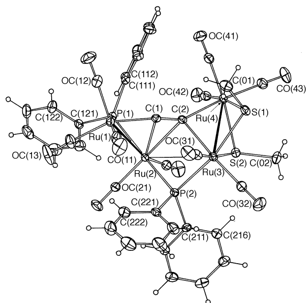
Fig. 2 Plot of a molecule of [\text{Ru}_4(\mu_4\text{-C}_2)(\mu\text{-SMe})_2(\mu\text{-PPh}_2)_2(\text{CO})_{10}] 3 showing the atom numbering scheme
